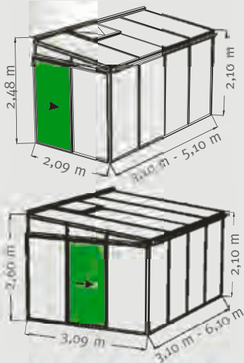
Viola II & III 1 line = 0,50 m Verglasungsraster
